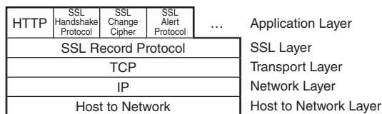
Figure 17.3 SSL adds an additional layer to the protocol stack as well as application layer protocols for controlling its own operation.
