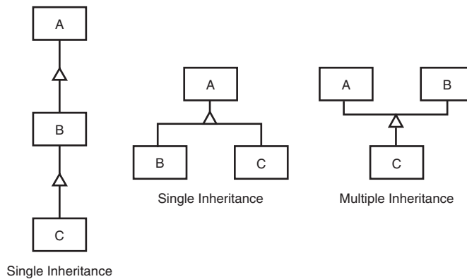
Figure 6.1 PHP does not support multiple inheritance.
