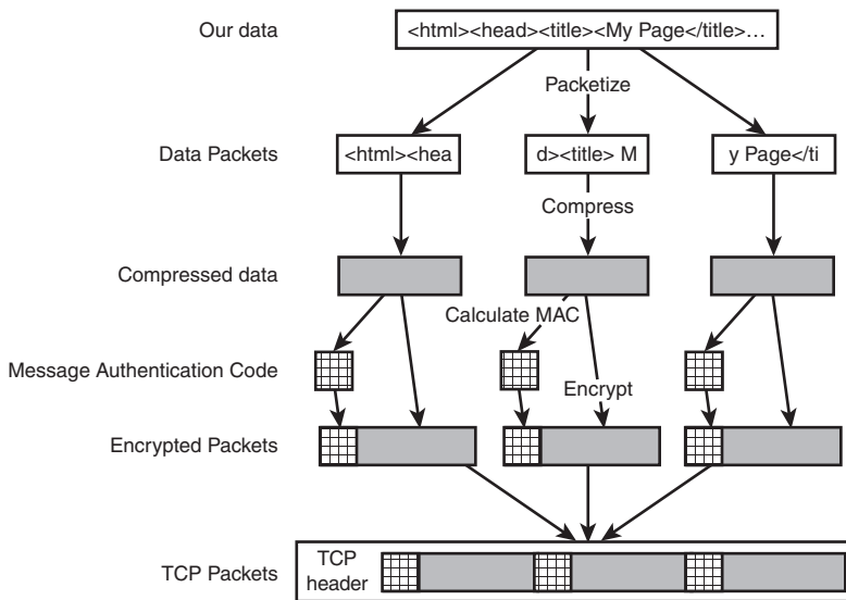
Figure 17.4 SSL breaks up, compresses, hashes, and encrypts data before sending it.
