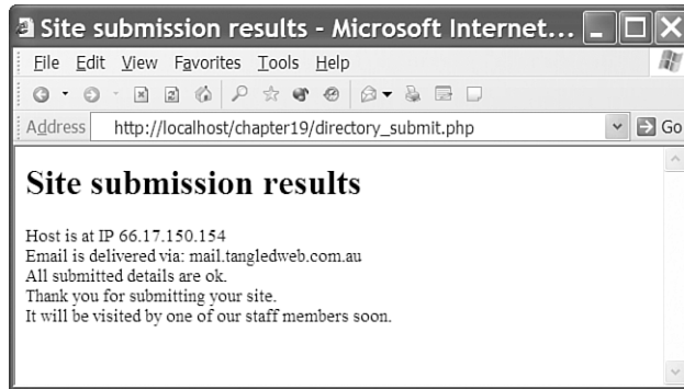
Figure 19.3 This version of the script displays the results of checking the hostnames for the URL and email address; a production version might not display these results, but it is interesting to see the information returned from the checks.
