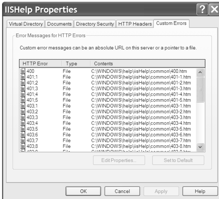
Figure 16.7 The Custom Errors tab lets you associate custom error pages with error events.
